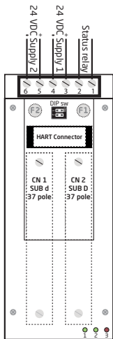
BACKPLANE DUAL CONNECTORS
